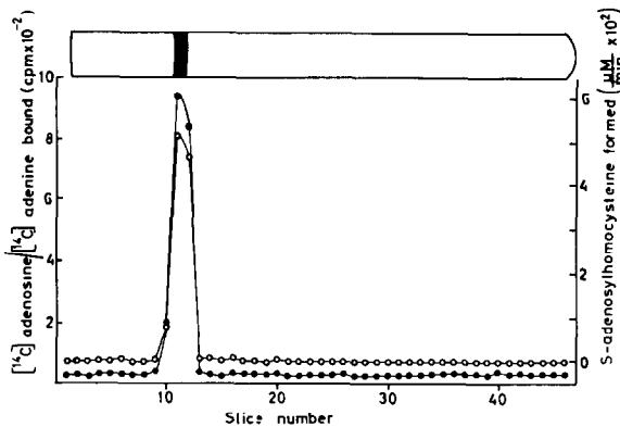
Fig. 2. Polyacrylamide gel electrophoresis of the native binding protein. Binding protein (40 \mu\text{g} ) was subjected to polyacrylamide gel electrophoresis at pH 8.8 and 9% gel. The gels were either stained or cut with a gel cutter. The gel slices were eluted and the binding of adenosine/adenine ( \bullet\text{--}\bullet ) measured as in [12]. The S -adenosylhomocysteine synthase activity ( \circ\text{--}\circ ) was determined at a 600-fold dilution of the eluate.
